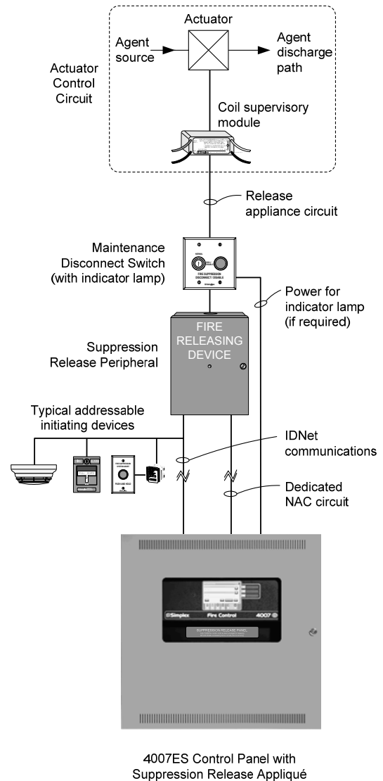
4007ES Series Releasing Control Typical Block Diagram
